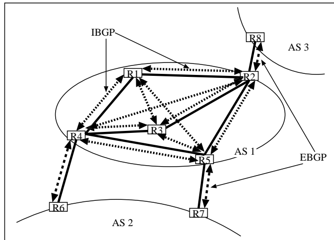
Figure 1: iBGP and eBGP
